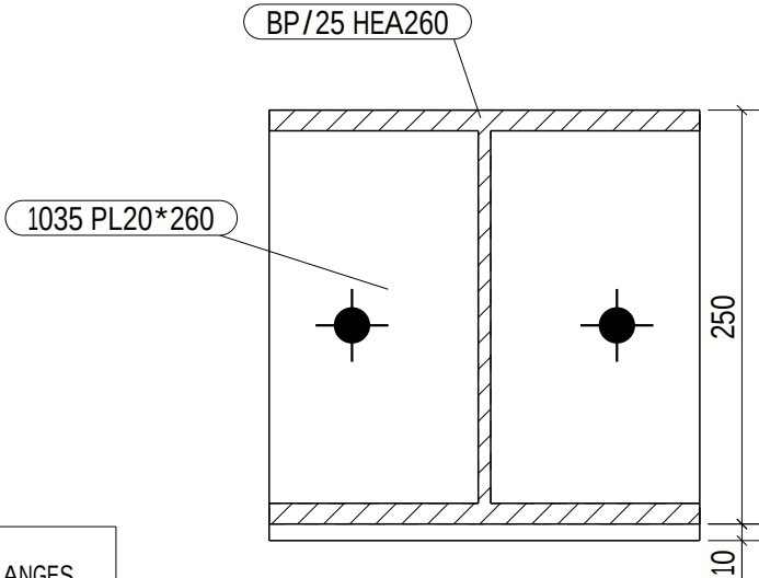
A - A 1:5
